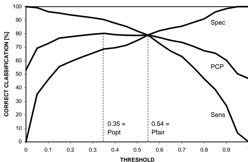
Figure 7.4. Estimation of the cut-off values based on P_{opt} (0.35) and P_{fair} (0.54). Percentage of correct prognoses (PCP) of the total model, sensitivity (Sens) and specificity (Spec) classification in relation to the threshold.
