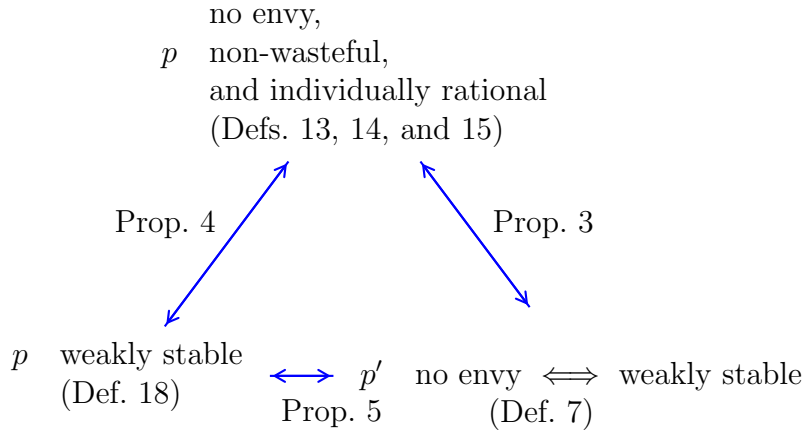
Figure 1: Relations between weak stability, no envy, non-wastefulness, and individual rationality for generalized deterministic matchings.
