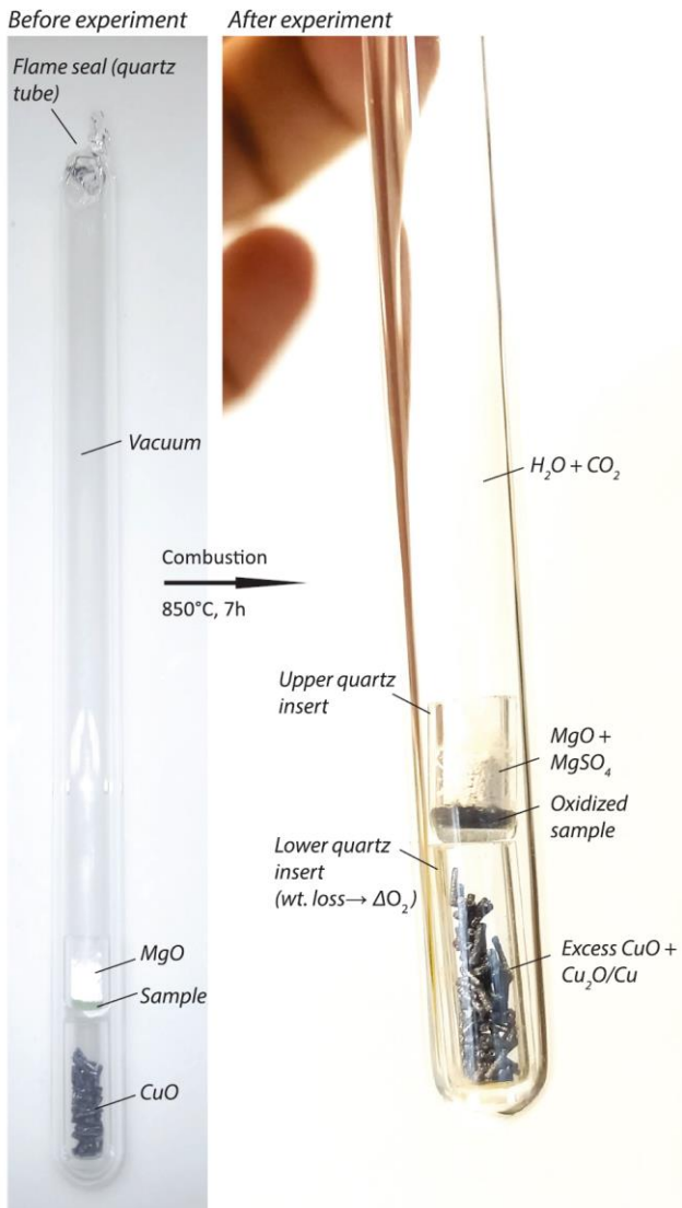
Fig. 1. Design of experimental assembly
